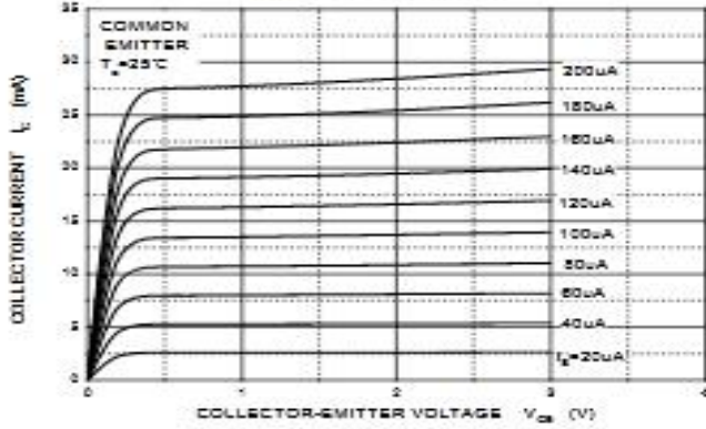
Static Characteristic
